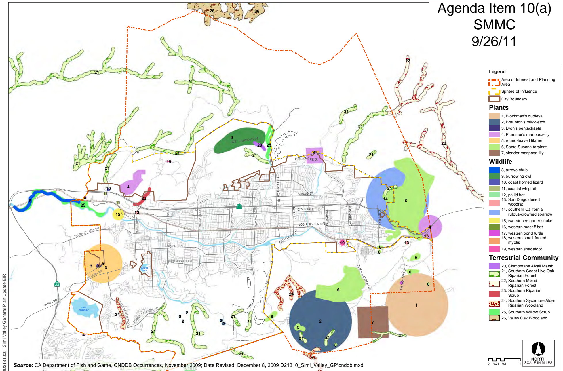
Figure 4.4-2 Sensitive Biological Resources within the Planning Area
